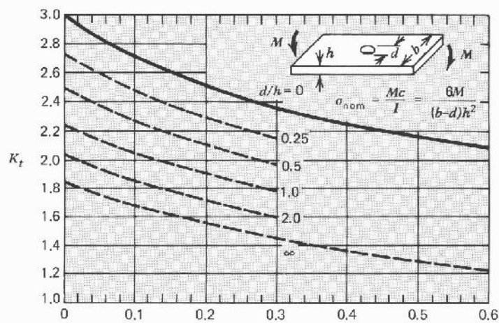
Figure 4.40 Plate with central hole (a) bending
