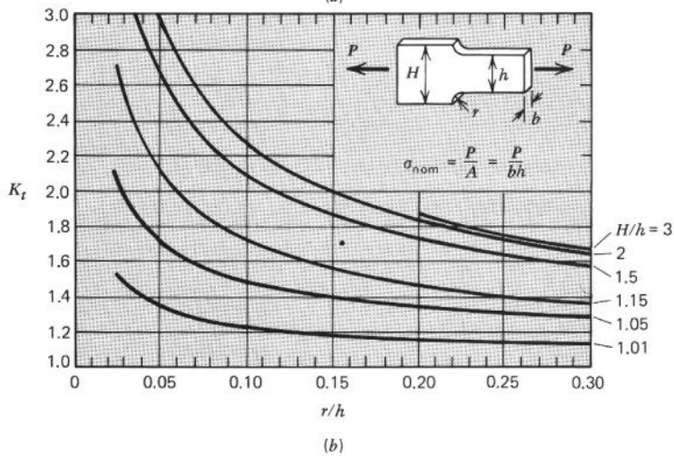
Figure 4.38 Bar with shoulder fillet (a) bending; (b) axial load [7].
