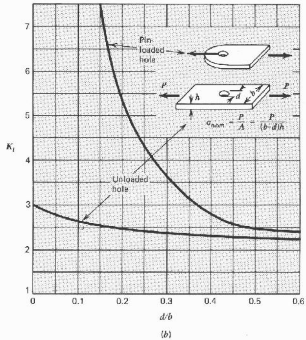
Figure 4.40 Plate with central hole (a) bending [7]; (b) axial hole [10].
