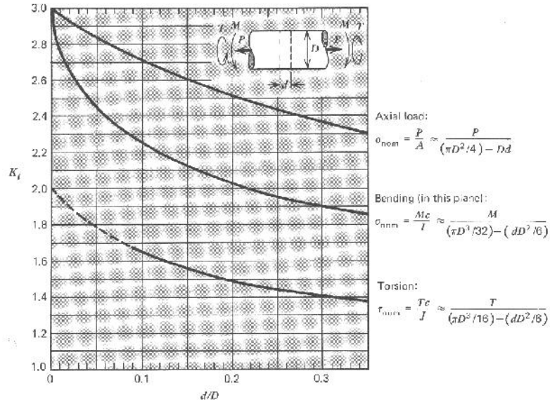
Figure 4.37 Shaft with radius hole [7].
