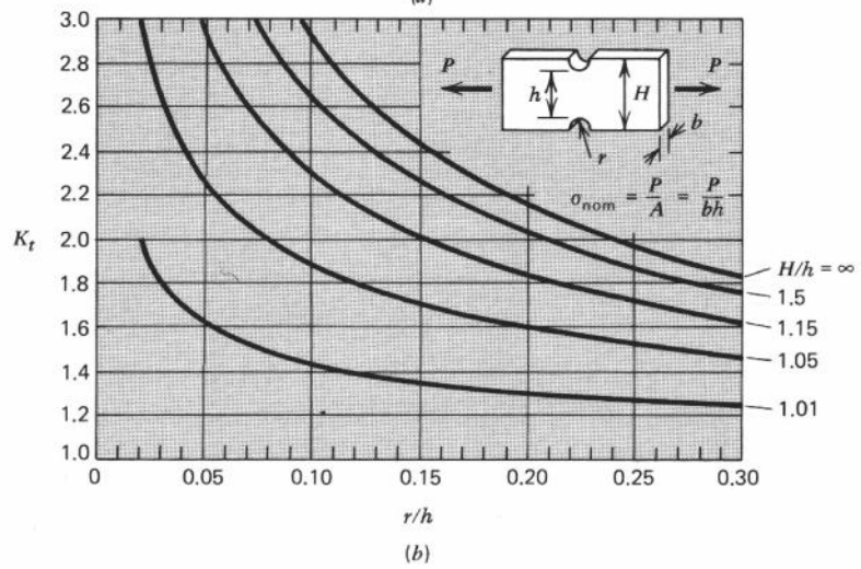
Figure 4.39 Notched flat bar (a) bending; (b) tension [7].
